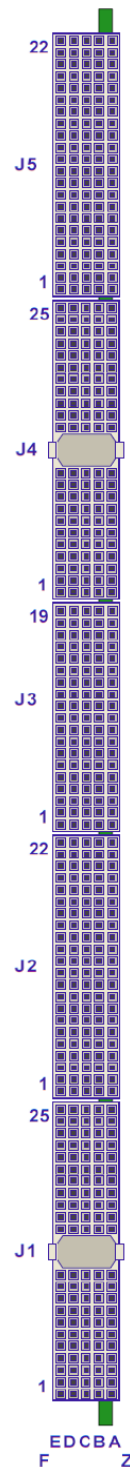
Figure 7: Compact PCI Connectors
